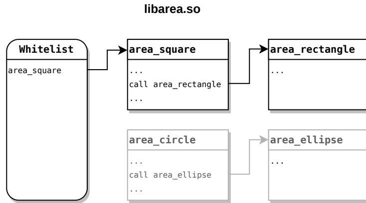
Fig. 1: Example of the basic idea of the analysis. A target application uses the function area_square . Hence, the function area_rectangle is also added to the whitelist.
